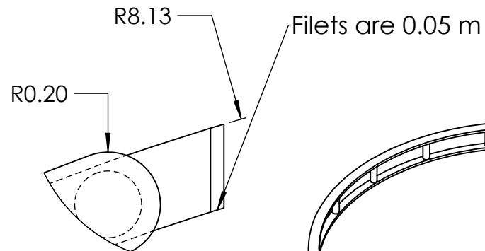
DETAIL A SCALE 1 : 20
